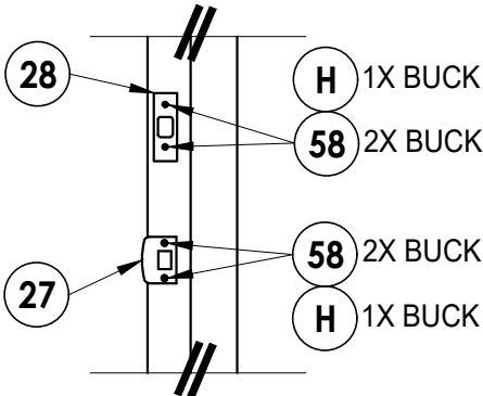
LATCH & DEADBOLT DETAIL
