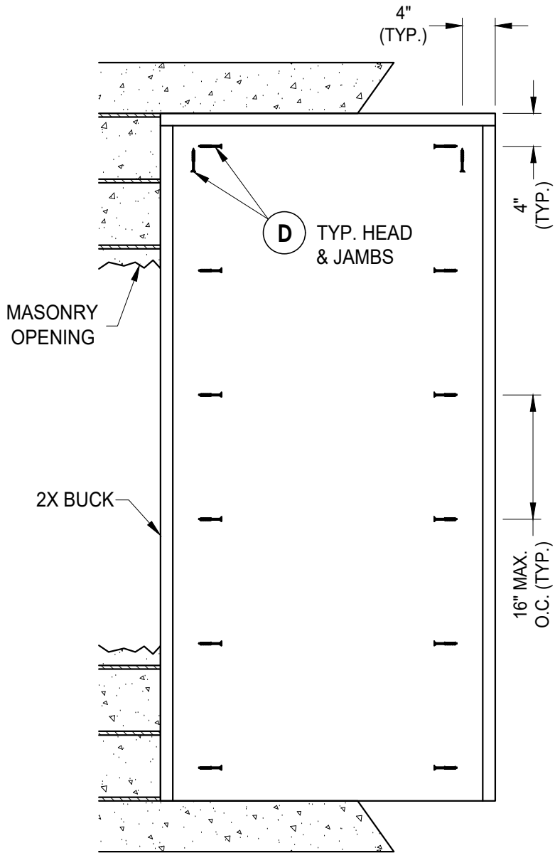
BUCK ANCHORING
